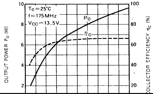
OUTPUT POWER, COLLECTOR EFFICIENCY VS. INPUT POWER
