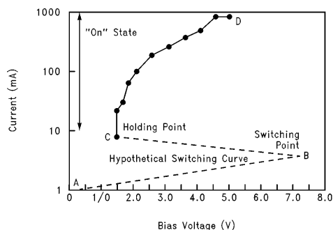
FIGURE 8. Latchup Condition for AT22V10B
