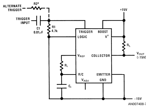
FIGURE 6. Operating Off Dual Supplies
