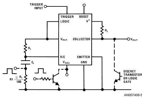
FIGURE 4. Cycle Interrupt
