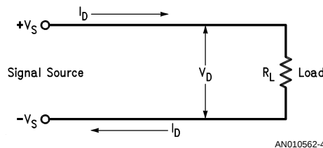
FIGURE 2. Differential-Mode Interference
