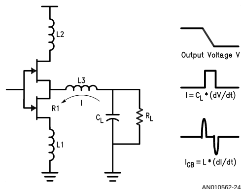
FIGURE 19. Ground Bounce
