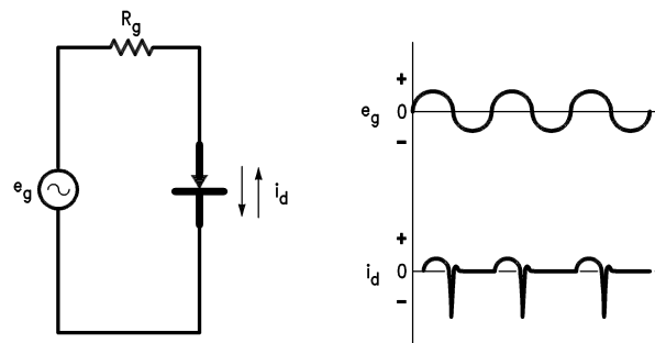
FIGURE 8. Diode Recovery Periods and Spikes
