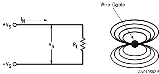
FIGURE 4. Field-to-Cable Coupling
