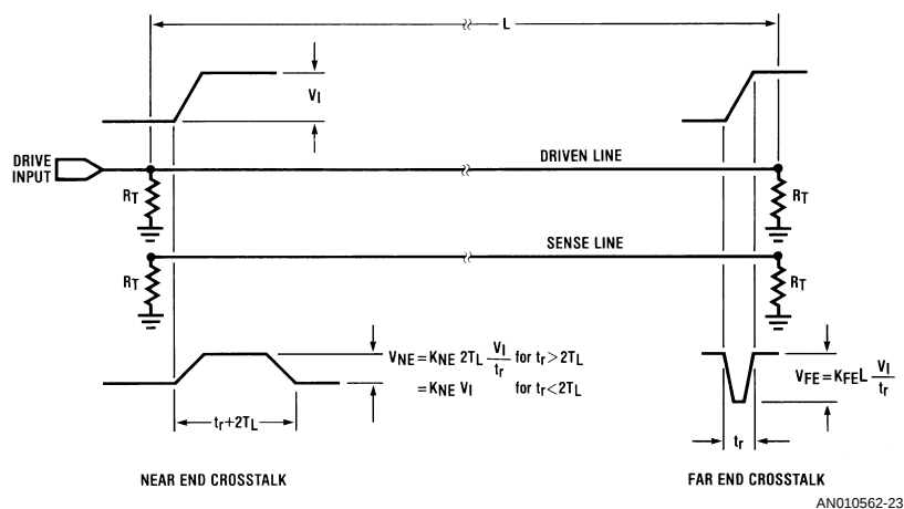
FIGURE 18. Crosstalk
