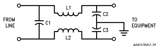
FIGURE 21. Filtering
