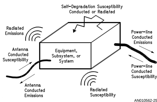
FIGURE 20. Intra-System EMI Manifestations
