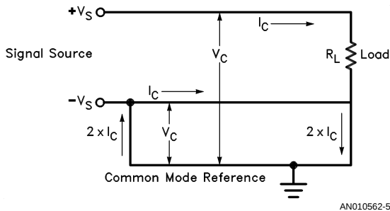
FIGURE 3. Common-Mode Interference
