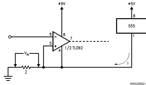
FIGURE 6. Common-Mode Impedance Coupling
