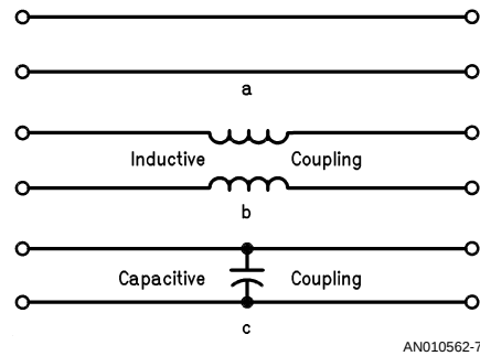
FIGURE 5. Cable-to-Cable Coupling
