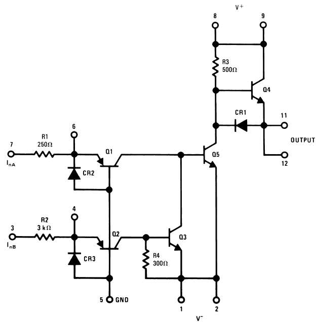
FIGURE 5. DH0035 Schematic Diagram
