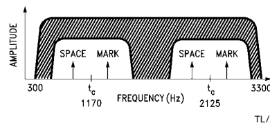
FIGURE 2. The HC942 modem chip converts incoming ones and zeros to mark and space frequencies when digital data enters the chip's TXD input
