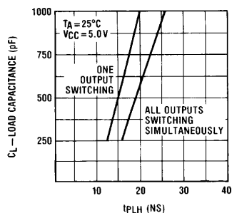
FIGURE 6a. t_{PLH} Measured to 2.7V on Output vs. C_L
