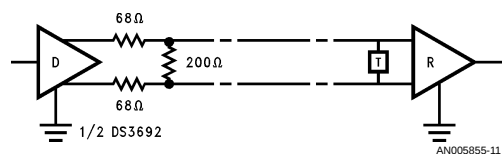
FIGURE 13. MIL STD 188-114A Balanced, Type 1 Typical Application
