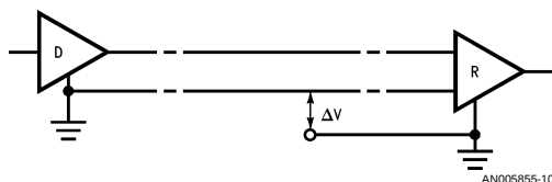
FIGURE 12. MIL STD 188-114A Unbalanced Typical Application
