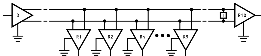
FIGURE 8. Typical TIA/EIA-422-B MultKdrop Application
