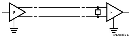
FIGURE 14. MIL STD 188-114A Balanced, Type 2 Typical Application
