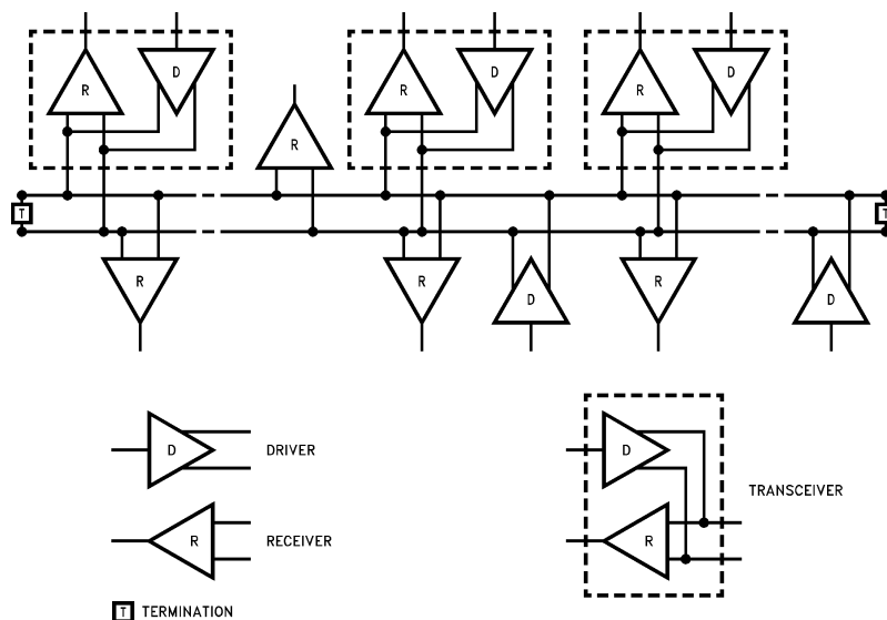
FIGURE 9. Typical TIA/EIA-485-A Application
