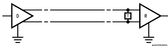
FIGURE 7. Typical TIA/EIA-422-B Point-to-Point Application
