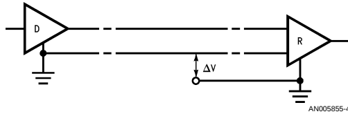
FIGURE 4. Typical TIA/EIA-423-B Application
