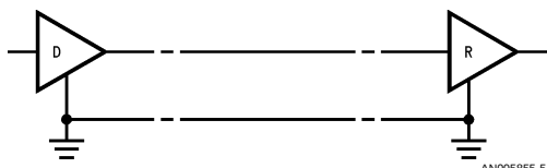
FIGURE 6. Typical TIA/EIA-694 Application
