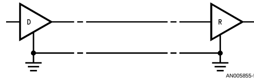
FIGURE 5. Typical TIA/EIA-562 Application
