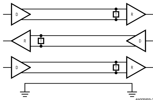
FIGURE 2. Balanced Data Transmission- 3 Channel, 7 Line and Ground
