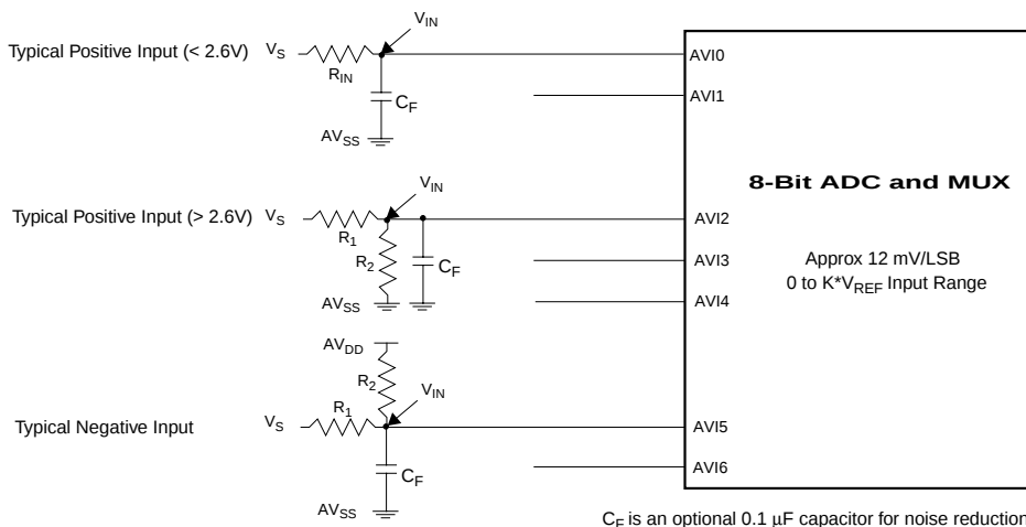
Figure 2. Analog Input Examples
