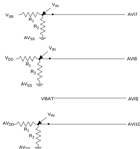
Figure 3. Internal Voltage Measurement
