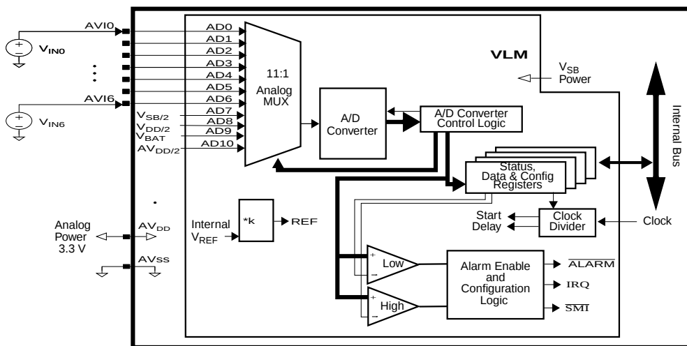
Figure 1. VLM Block Diagram
