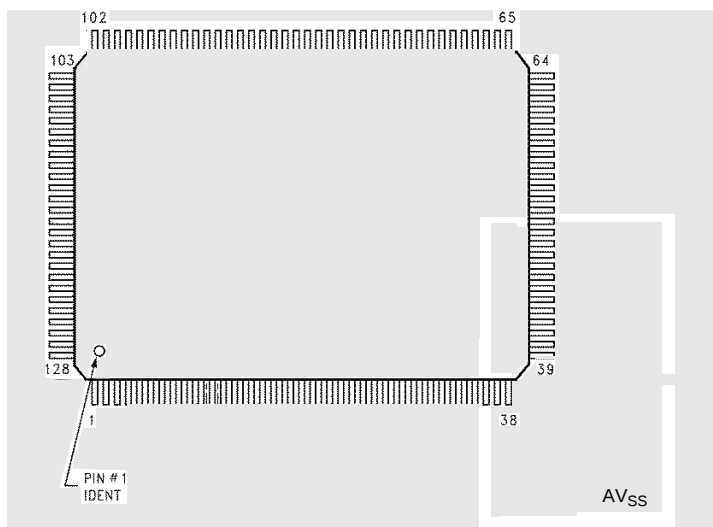
Figure 5. AV_{SS} Plane Layout Example
