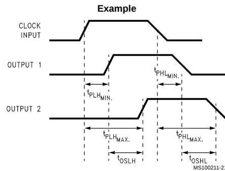
FIGURE 13. t_{OSLH} , t_{OSHL}
