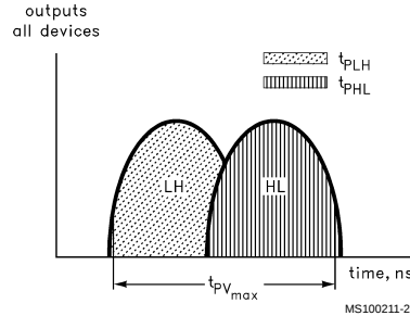
FIGURE 19. t_{PV}
