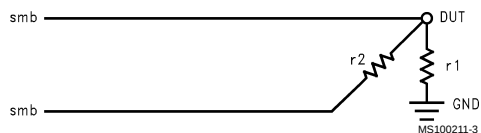
FIGURE 38. Input
