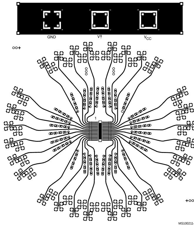
FIGURE 36. 28-Pin SOIC TOP (Viewed from Top)
