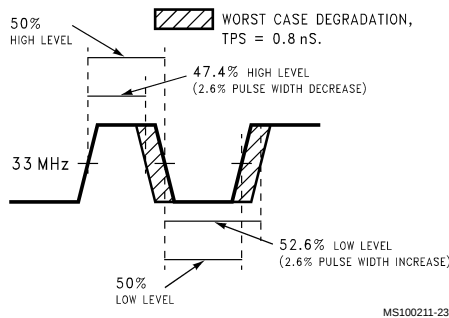
FIGURE 15. Pulse Width Degradation
