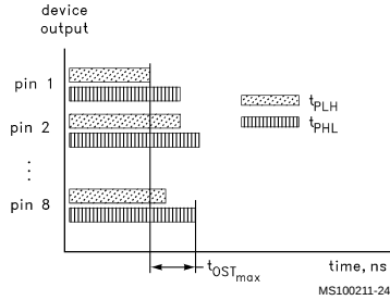
FIGURE 16. t_{OST}
