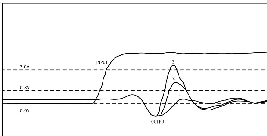
FIGURE 31. V_{ILD} 7 Outputs Switching V_{CC} = 5.0V , T_A = 25^\circ C
