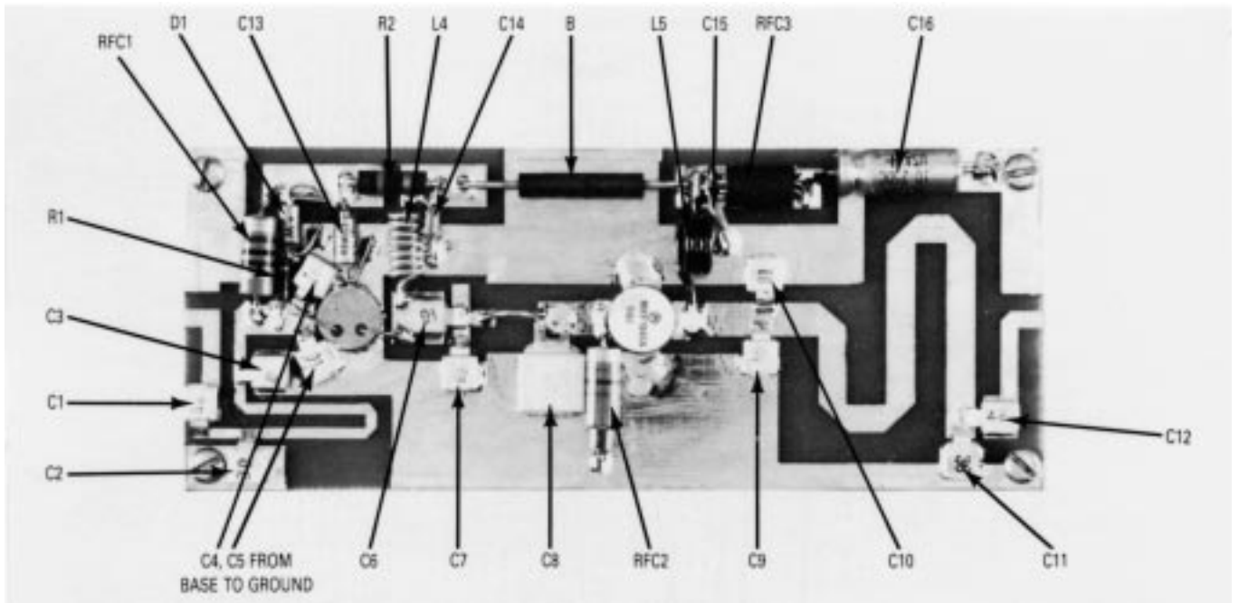
Figure 3. Parts Placement
