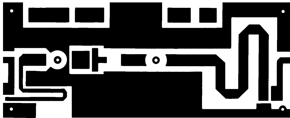
Figure 4. PCB Photomaster
