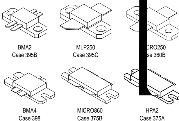
Figure 1. Example of CuW Packages
