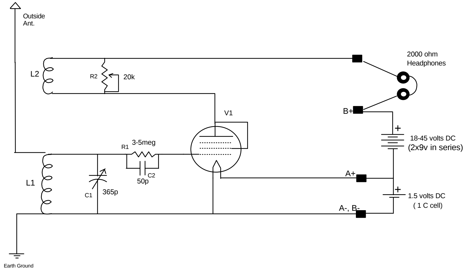
Circuit 2
