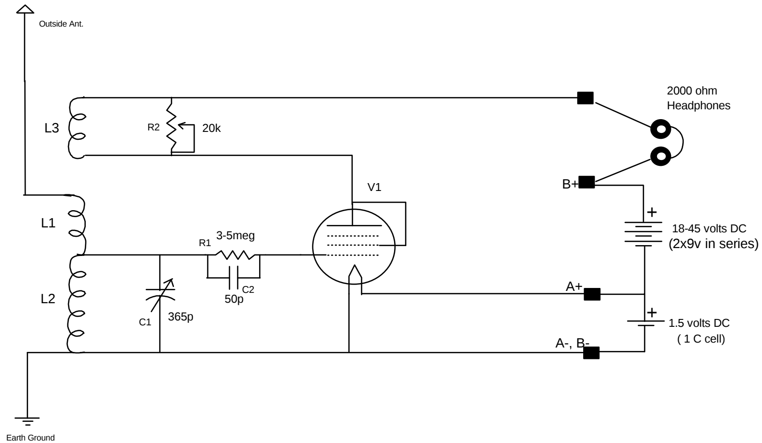
Circuit 1
